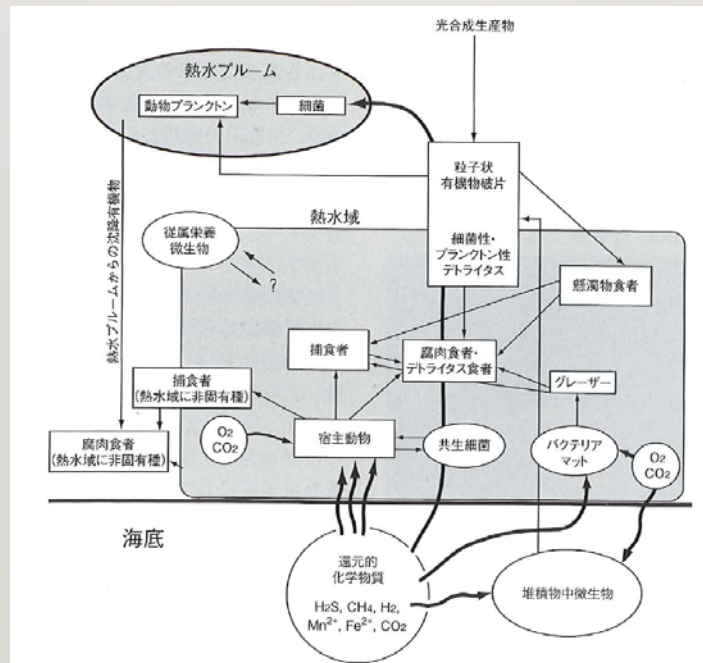
Fig. 2.16. 熱水噴出域における栄養段階のダイアグラム. Tunnicliffe (1991)を改変. The trophic interactions diagram of a hydrothermal vent ecosystem. Modified from Tunnicliffe (1991).
